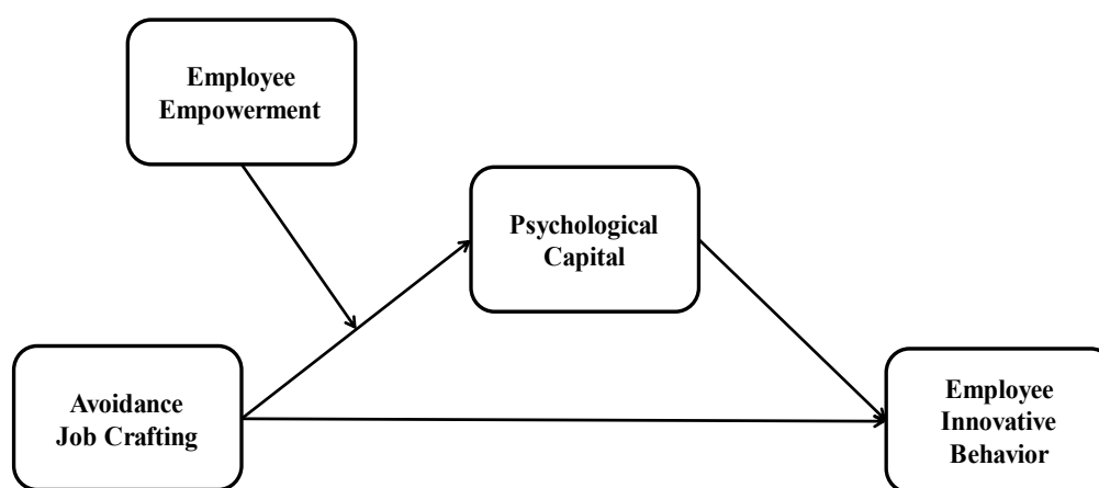
Figure 1: Hypothesized Model
