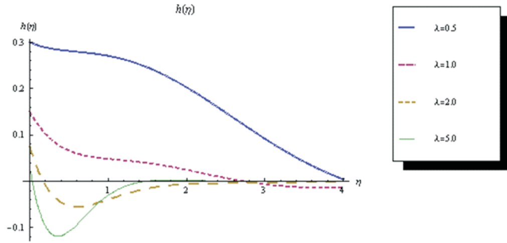
FIGURE 9. The variation of \lambda and K on h(\eta) , K = 0.3
