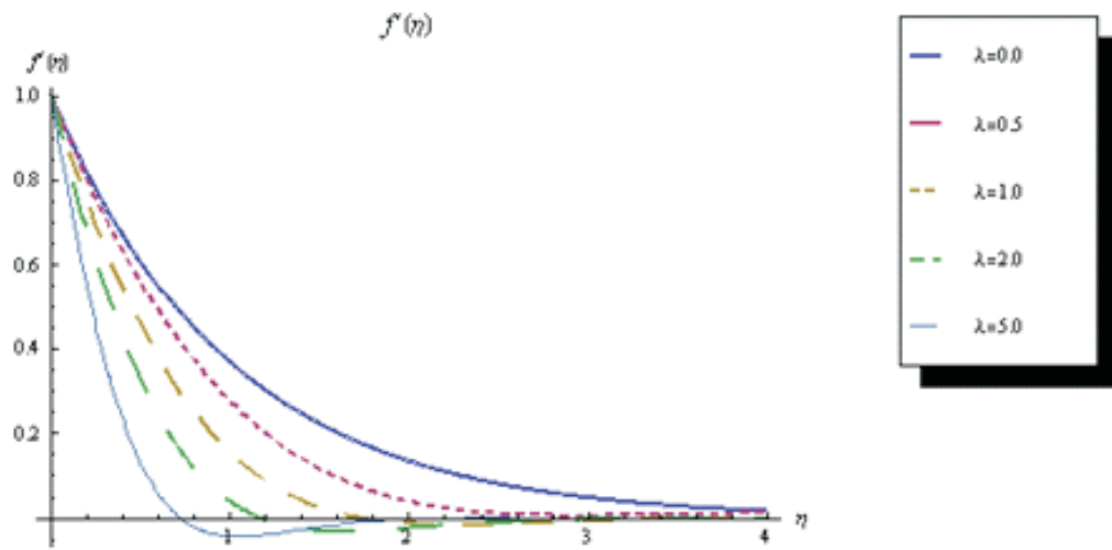
FIGURE 5. The variation of \lambda and K on f'(\eta) , K = 0.0
