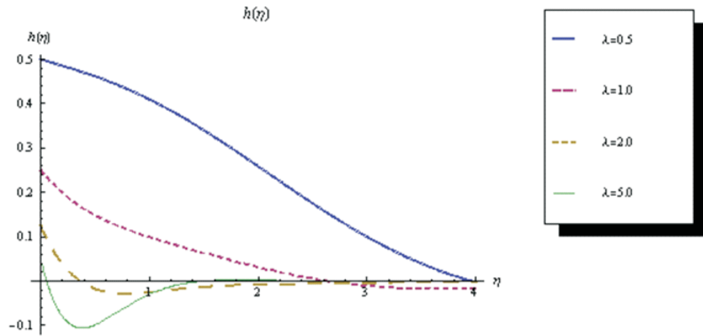
FIGURE 7. The variation of \lambda and K on h(\eta) , K = 0.0
