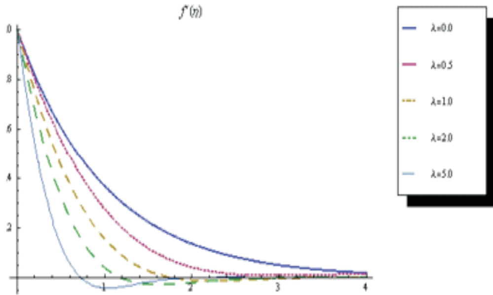
FIGURE 5. The variation of \lambda and K on f'(\eta) , K = 0.0
