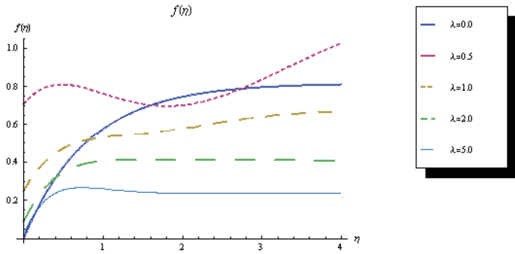
FIGURE 3. The variation of \lambda and K on f(\eta) , K = 0.1
