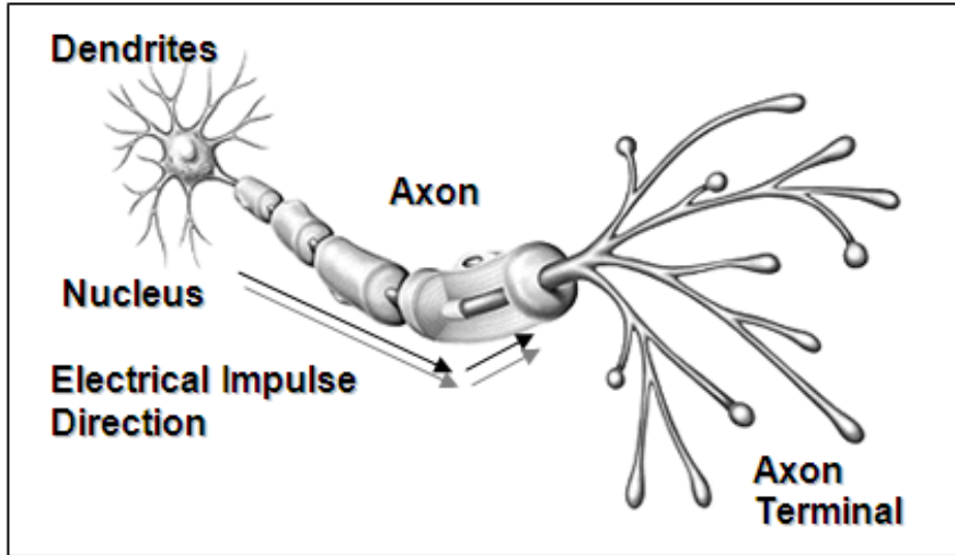
FIGURE 1 Biological Model of Human Neuron
